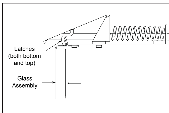
Figure 4.1 Glass Assembly
