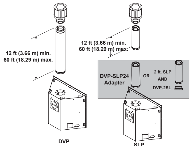
Figure 4.10 DVP-SLP24 Adapter
