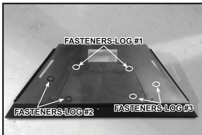
Figure 2. Log Fastener Locations on Base Pan
