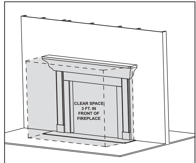
Figure 3.1 Clear Space Requirement
