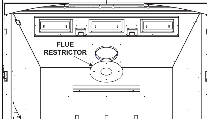
Figure 4.10 Flue Restrictor Installation
