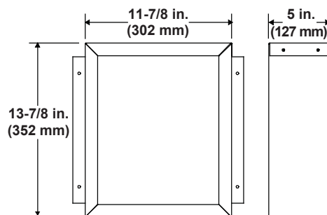
DVP-BE2 DVP-HPC Cap Brick Extension
