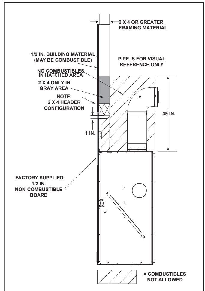
Figure 10.8 Non-Combustible Zone
