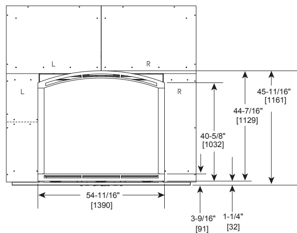
ARCHED FIRESCREEN
